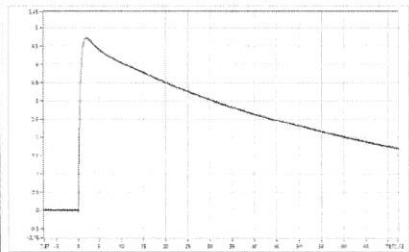
SP_011 Upk=4.72 kV; T1=1.09 us; T2=48.83 us; Beta'=3.77 %;
