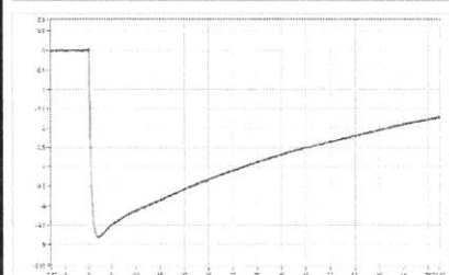
SN_014 Upk=-4.80 kV; T1=1.10 us; T2=48.79 us; Beta'=3.57 %;
