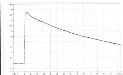
SP_009 Upk=4.74 kV; T1=1.09 us; T2=48.70 us; Beta'=3.83 %;
