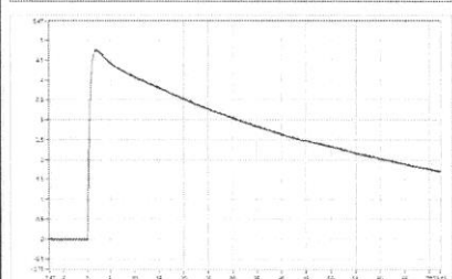
SP_014 Upk=4.73 kV; T1=1.09 us; T2=48.76 us; Beta'=3.87 %;
