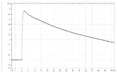
SP_025 Upk=4.80 kV; T1=1.09 us; T2=48.53 us; Beta'=3.75 %;
