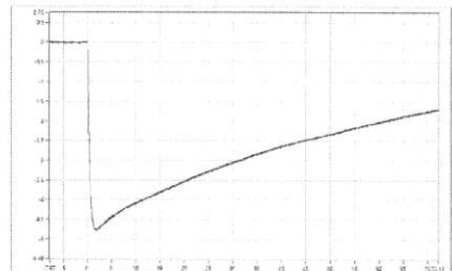
SN_013 Upk=-4.74 kV; T1=1.09 us; T2=48.57 us; Beta'=3.87 %;
