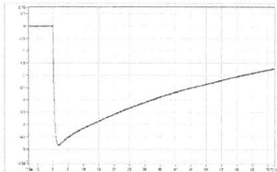
SN_012 Upk=-4.83 kV; T1=1.09 us; T2=48.55 us; Beta'=3.75 %;
