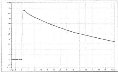
SP_008 Upk=4.81 kV; T1=1.08 us; T2=48.54 us; Beta'=4.11 %;
