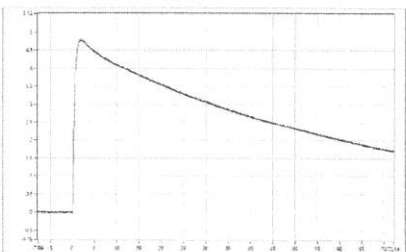
SP_013 Upk=4.77 kV; T1=1.09 us; T2=48.63 us; Beta'=4.00 %;
