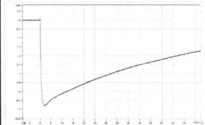
SN_011 Upk=-4.78 kV; T1=1.10 us; T2=48.95 us; Beta'=3.48 %;
