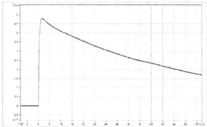
SP_022 Upk=4.78 kV; T1=1.09 us; T2=48.69 us; Beta'=4.13 %;
