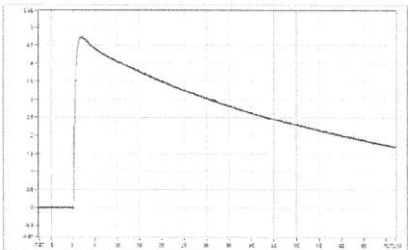
SP_023 Upk=4.71 kV; T1=1.09 us; T2=48.27 us; Beta'=3.99 %;
