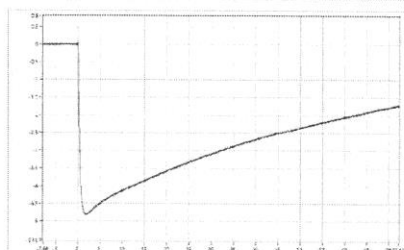
SN_020 Upk=-4.81 kV; T1=1.10 us; T2=48.80 us; Beta'=3.70 %;
