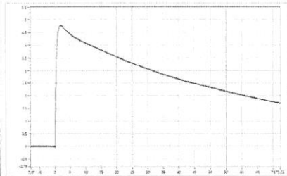
SP_021 Upk=4.76 kV; T1=1.09 us; T2=48.76 us; Beta'=3.94 %;
