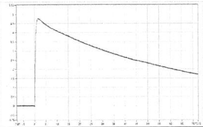
SP_007 Upk=4.75 kV; T1=1.09 us; T2=48.62 us; Beta'=3.98 %;
