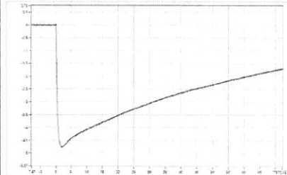
SN_016 Upk=-4.76 kV; T1=1.09 us; T2=48.51 us; Beta'=3.84 %;
