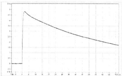
SP_012 Upk=4.80 kV; T1=1.09 us; T2=48.78 us; Beta'=3.78 %;
