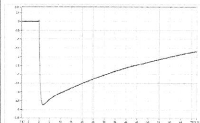
SN_019 Upk=-4.72 kV; T1=1.09 us; T2=48.79 us; Beta'=3.60 %;
