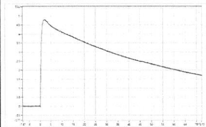
SP_024 Upk=4.78 kV; T1=1.09 us; T2=48.70 us; Beta'=3.85 %;
